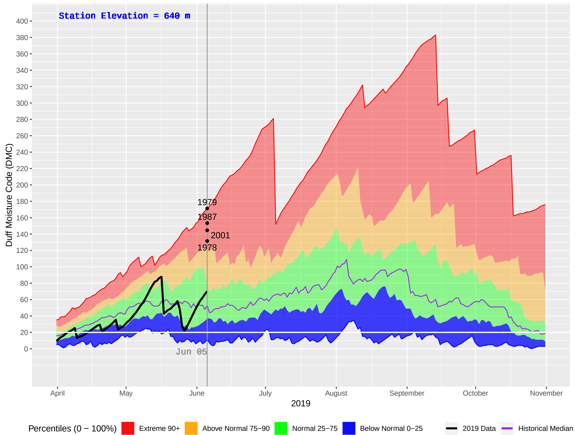
MERRITT HUB (294) : Historical (1978–2018), Current (2019) Daily Duff Moisture Code (DMC)
