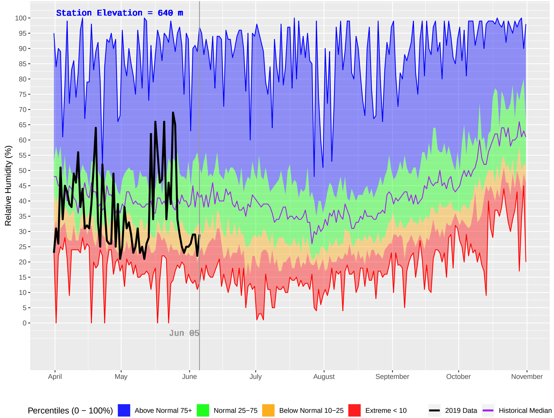
MERRITT HUB (294) : Historical (1978–2018) and Current (2019) Daily Relative Humidity
