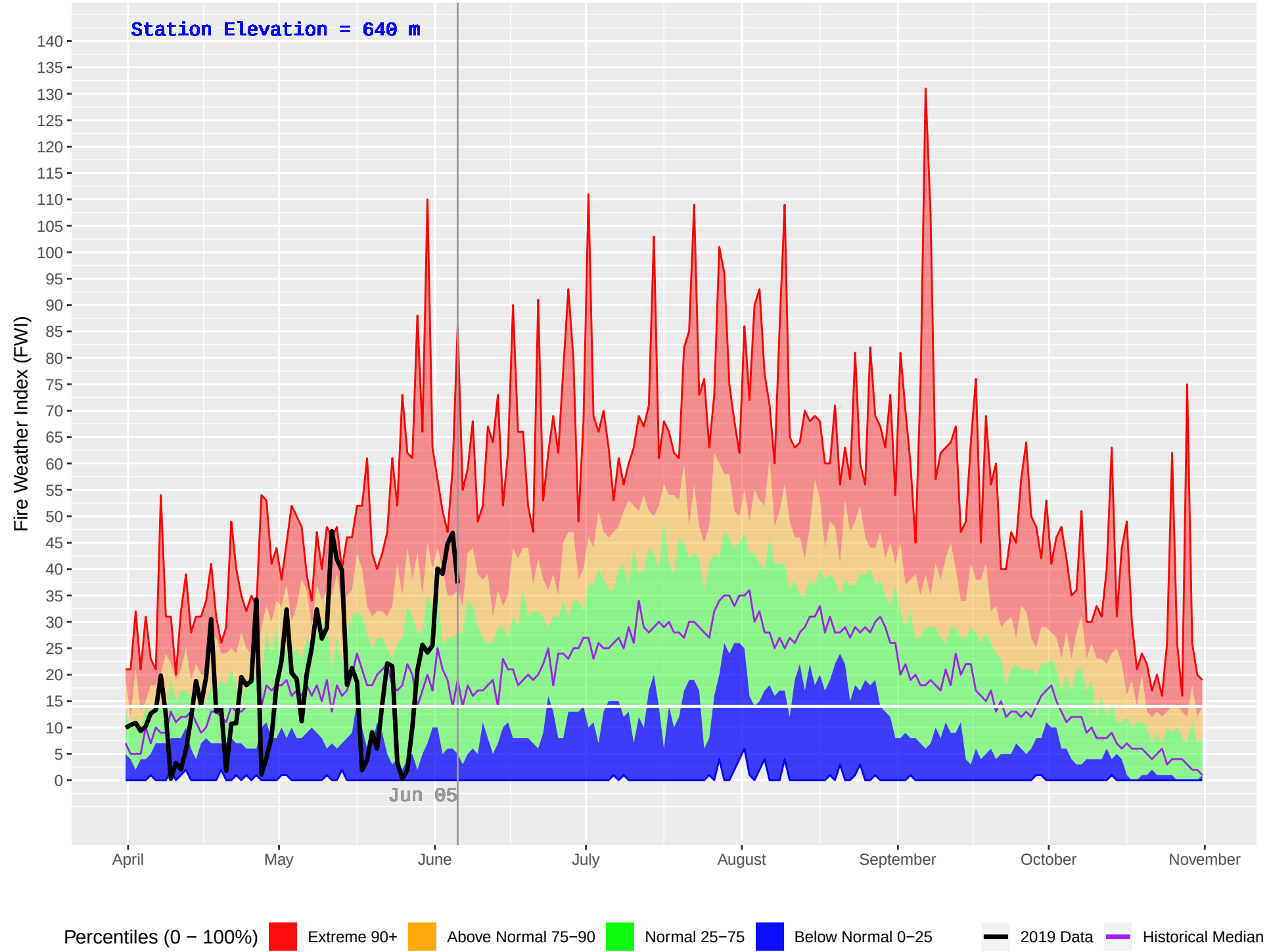
MERRITT HUB (294) : Historical (1978–2018) and Current (2019) Daily Fire Weather Index (FWI)
