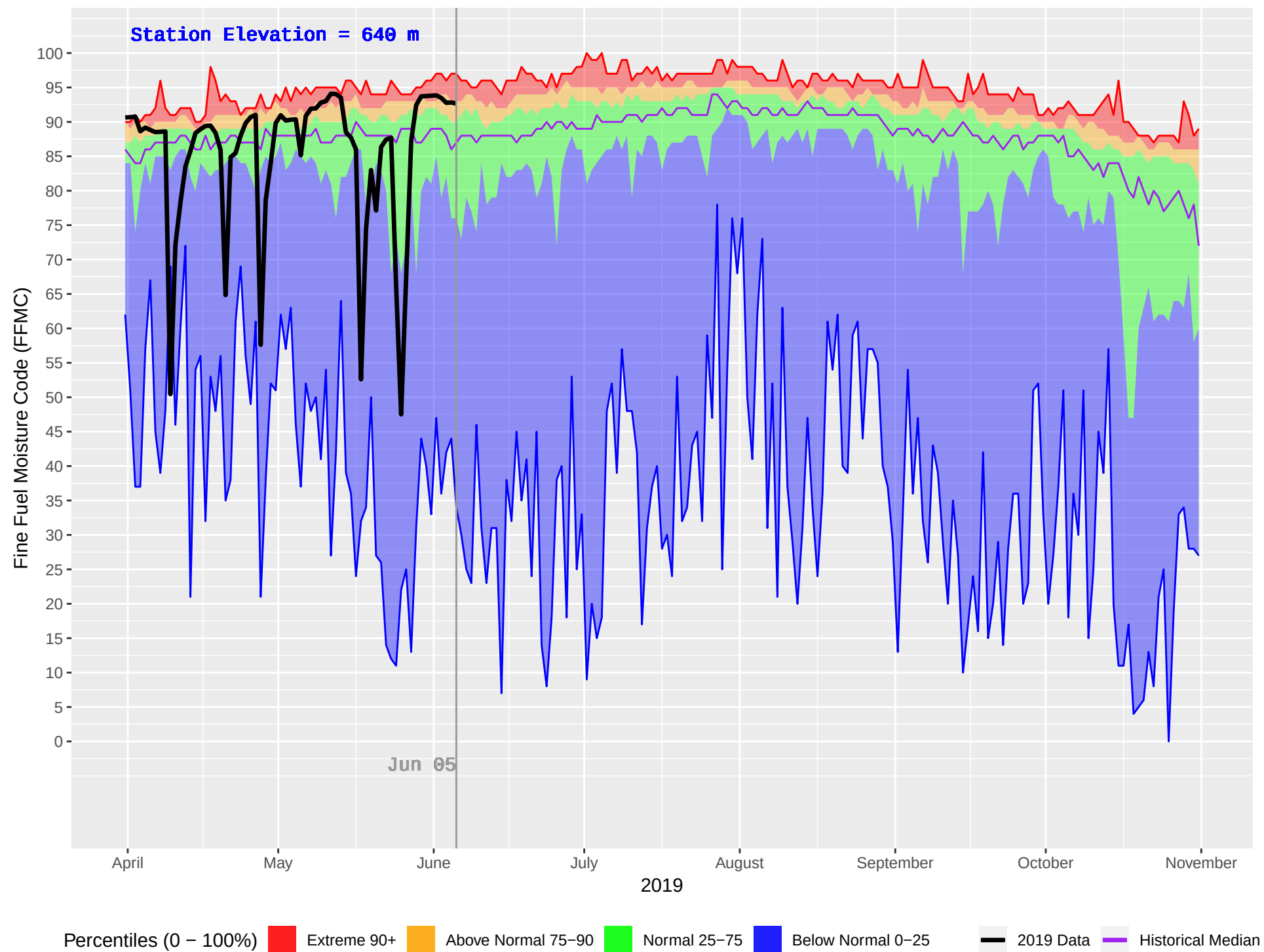
MERRITT HUB (294) : Historical (1978–2018) and Current (2019) Daily Fine Fuel Moisture Code (FFMC)
