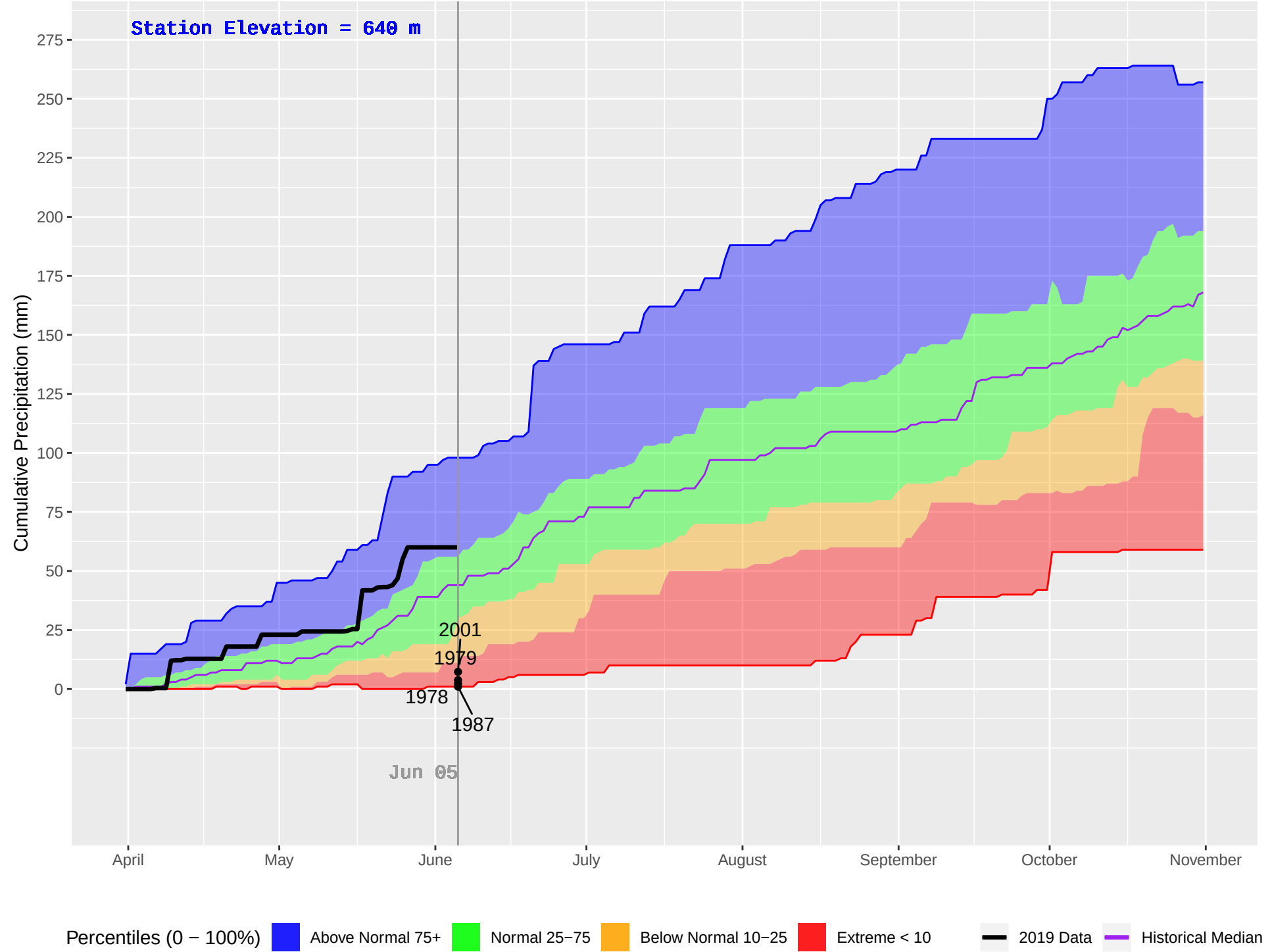
MERRITT HUB (294) : Historical (1978–2018), Current (2019) Daily Cumulative Precipitation
