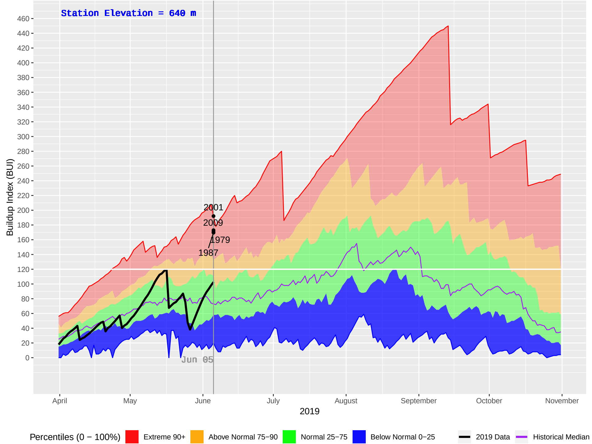
MERRITT HUB (294) : Historical (1978–2018), Current (2019) Daily Buildup Index (BUI)
